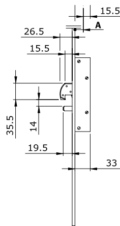
Deviator with rotating hook
