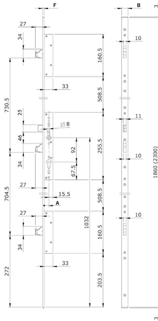
Deviator with rotating hook
